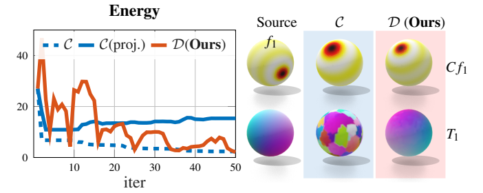
Figure 9: For the input descriptor (f_1, g_1) in Fig. 4, we compare our discrete solver ( \mathcal{D} ) to the continuous solver ( \mathcal{C} ). We visualize the transported descriptor and the recovered pointwise map on the right. See Fig. 15 and 16 in Appendix C for the corresponding results of the other two pairs of descriptors.
