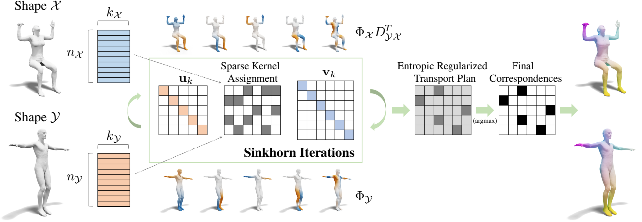
Figure 3: Fast Sinkhorn Filters: Illustrating spectral embedding alignment using regularized optimal transport. Our pipeline inputs a set of aligned basis functions and outputs a pointwise correspondence between the shapes.
